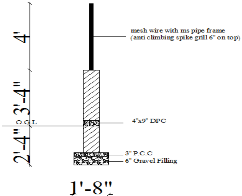
Wall Section
